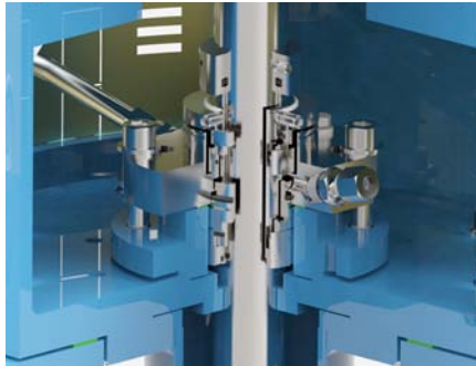
Single or double Cartridge seal
