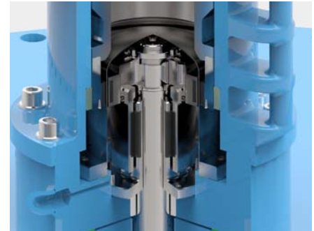
Seal less, magnetic drive
