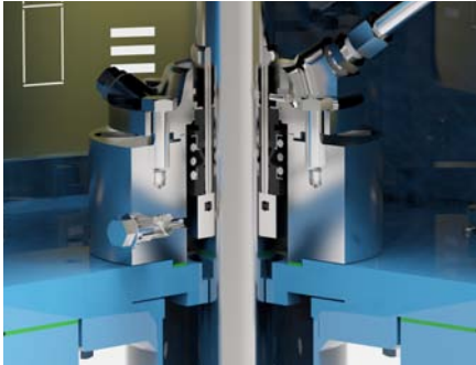
Mechanical seal EN 12756 (DIN 24960)
